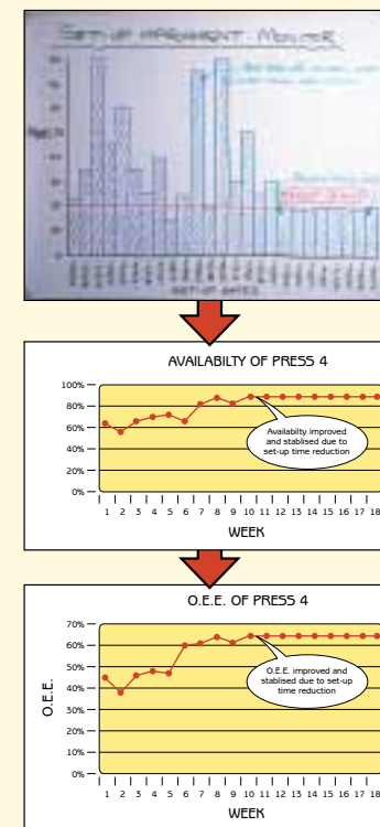
Figure 9 - Data monitoring set-up time and its effect on OEE.
